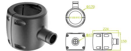
108 Holder
