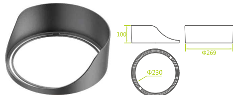
Rotatable diffuser
