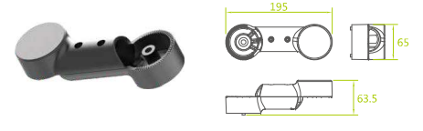
Extension supporter
