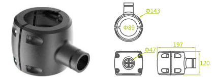
89 Holder
