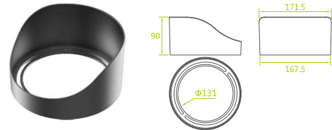
Rotatable diffuser
