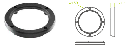
Standard Cover
