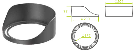
Rotatable diffuser
