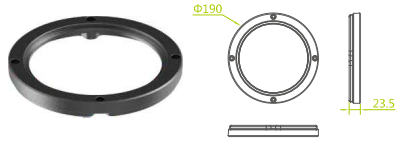
Standard Cover
