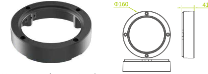
High cover(anti-glare)
