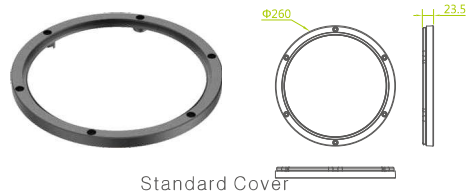
Standard Cover
