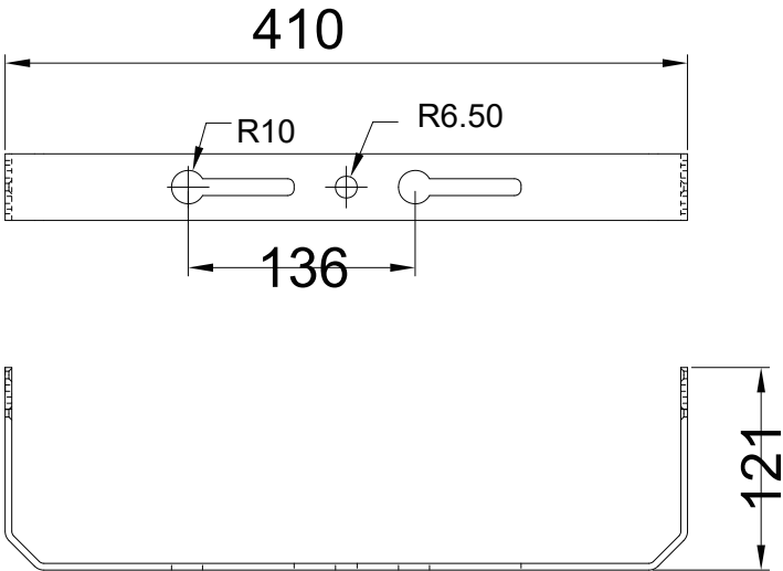
Bracket Detail
