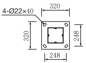
Flange Assembly
