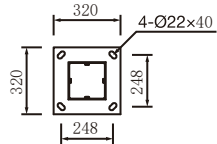
Flange Assembly
