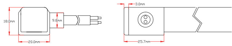
Connector Section
