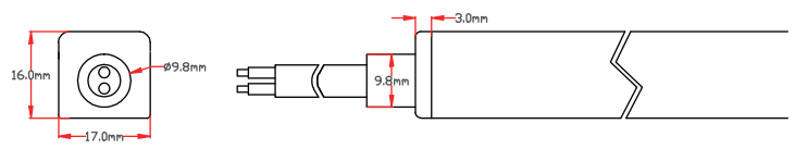
Connector Section
