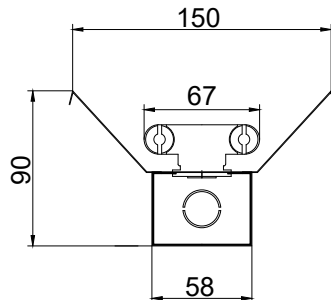
Twin Tube With Reflector
