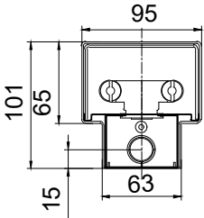
Twin / Single Tube
