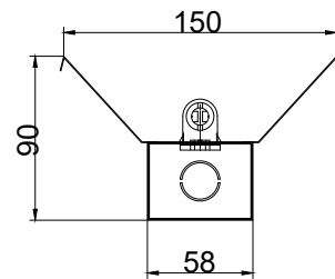
Single Tube With Reflector
