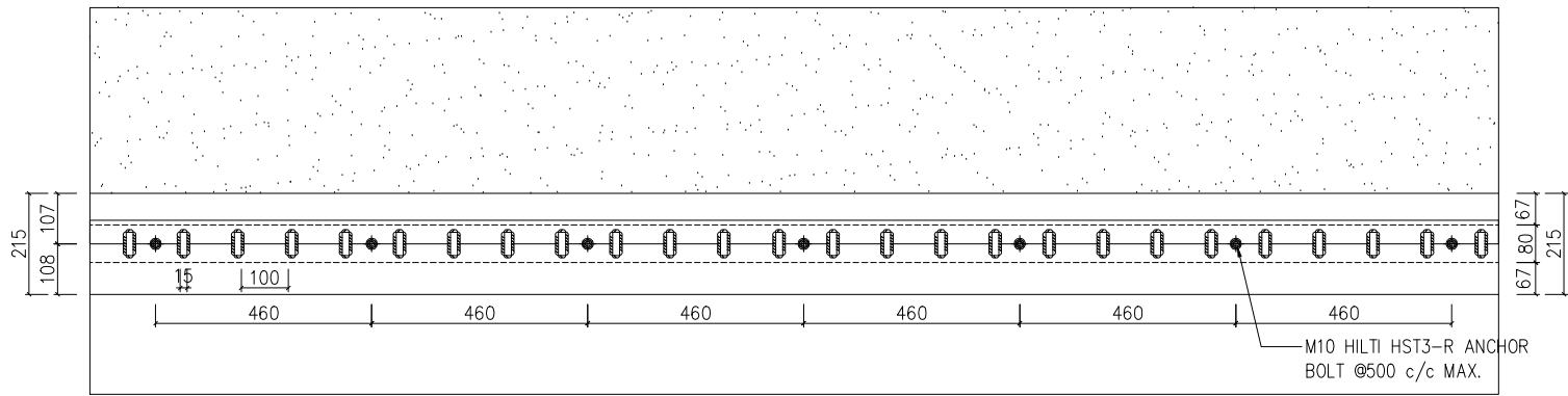
2 HANNAH@ FENCE 68 TYPICAL PLAN SCALE 1:8
