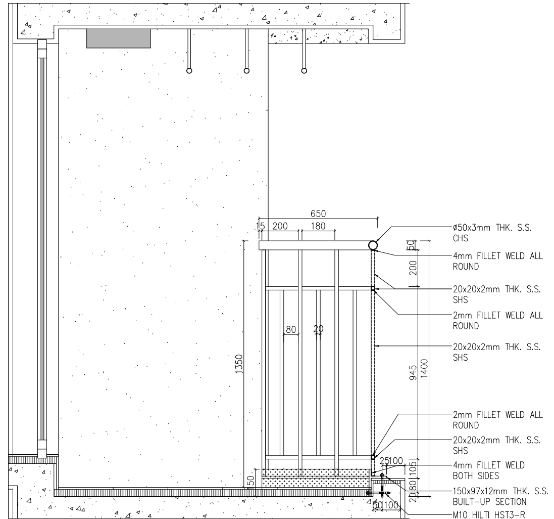
B HANNAH@FENCE 18 ELEVATION SCALE 1:10
