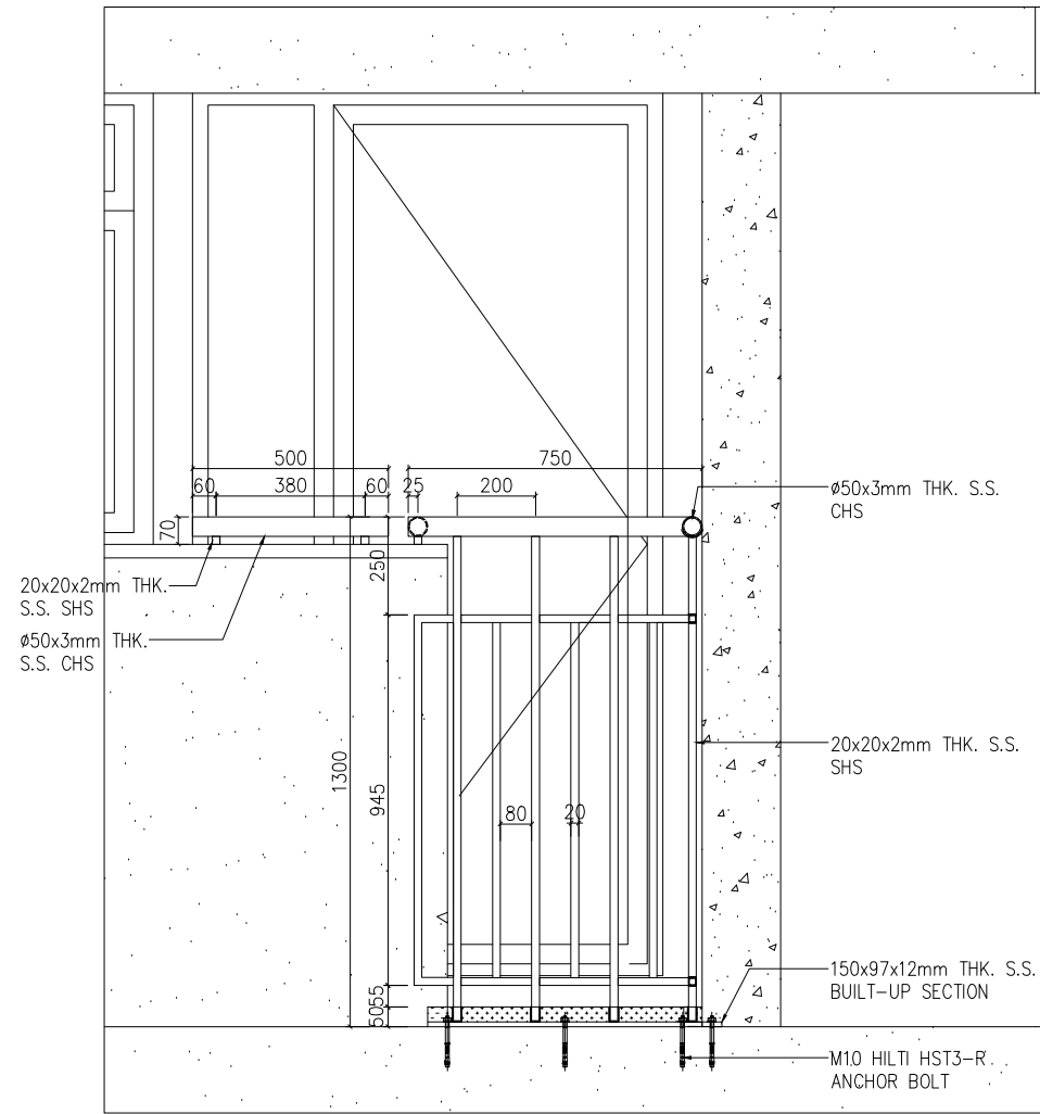
A HANNAH@FENCE 18 ELEVATION SCALE 1:10
