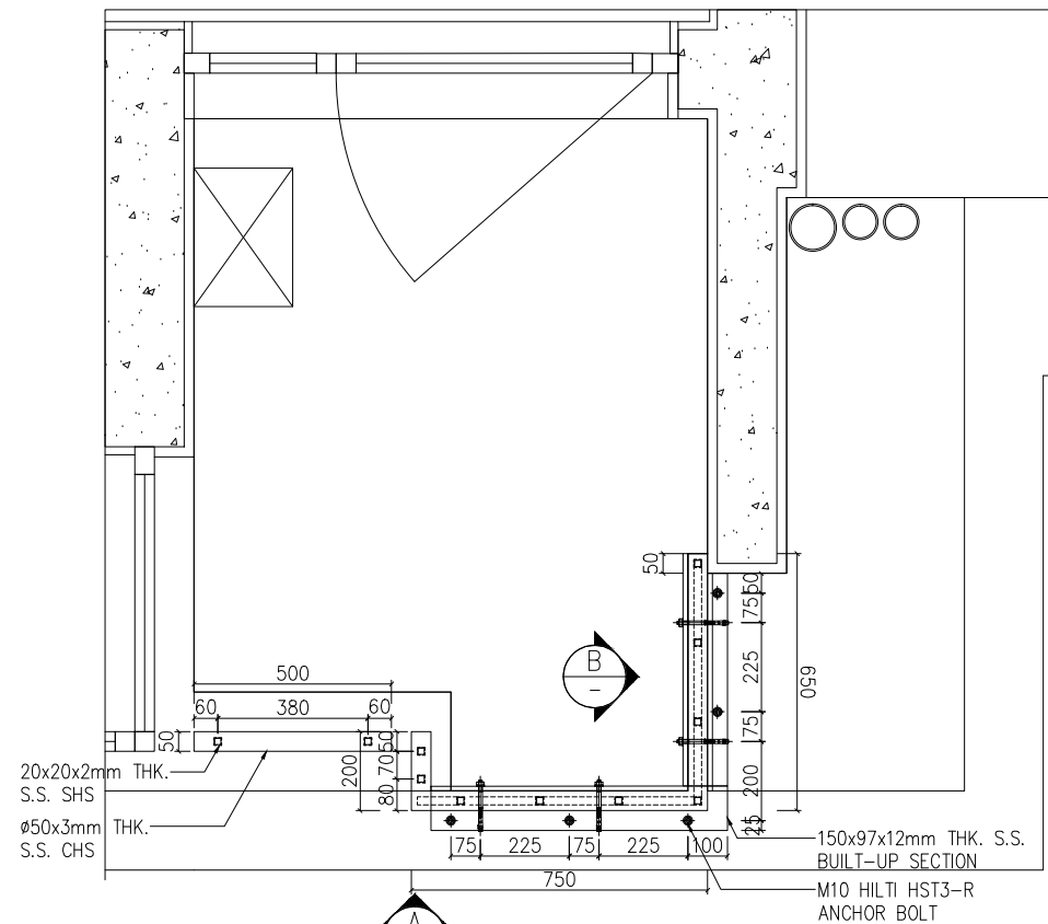
1 HANNAH@FENCE 18 PLAN SCALE 1:10
