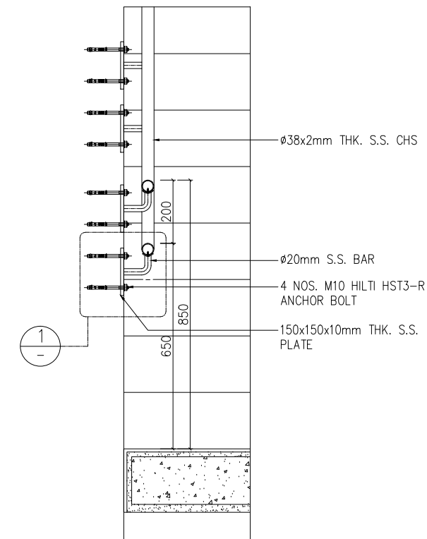
A SECTION SCALE 1:8
