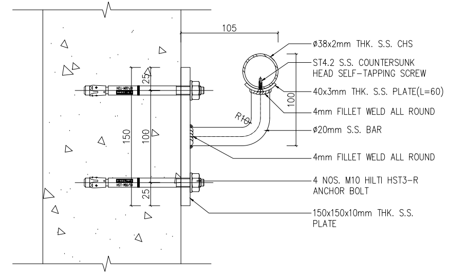
1 DETAIL SCALE 1:2
