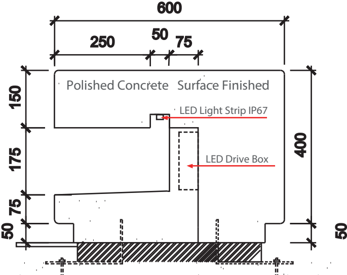
Type A (with LED Strip Light)
