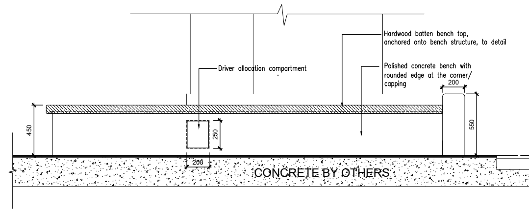
ELEVATION D
