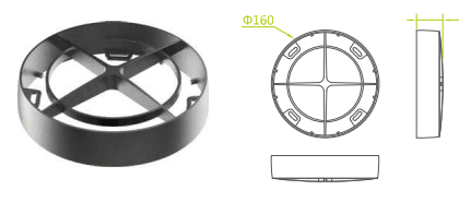
Star exterior anti-glare shield
