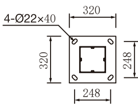
Flange Assembly
