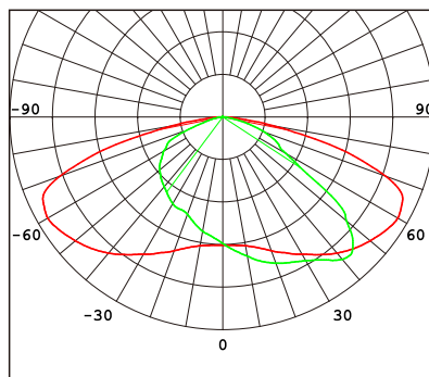
Type III Medium (94x158° Tilt45°) R00803
