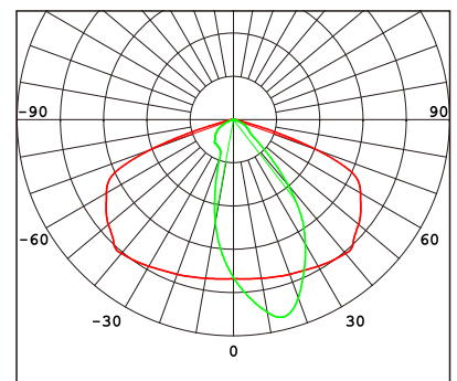
Type II Short (50x145° Tilt20°) R01609
