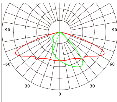
Type II Short (70x155° Tilt30°) R01606
