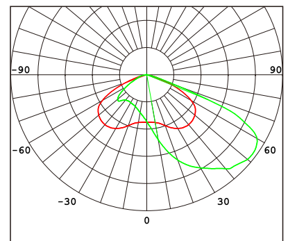
Type IV Very Short (58x139° Tilt55°) R00804
