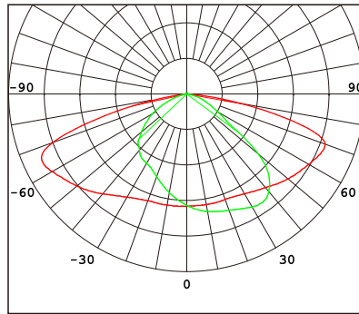
Type III Medium (96x157° Tilt40°) R02413
