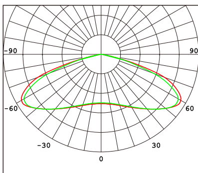
Type VS Short (150x150°) R00805
