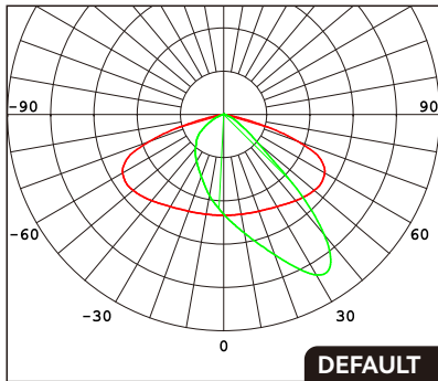
Type II Short (50x148° Tilt35°) R01610
