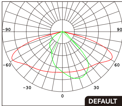
Type II Short (68x150° Tilt25°) R02411
