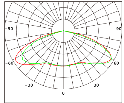
Type VS (150x150°) R02415
