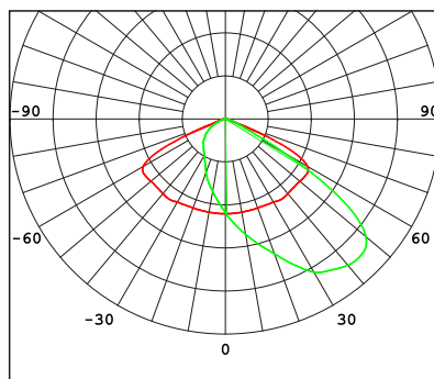
Type III Short (54x135° Tilt50°) R01607
