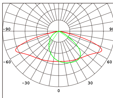
Type III Medium (94x157° Tilt35°) R01613
