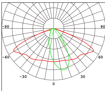
Type I Short (43x143° Tilt15°) R01601
