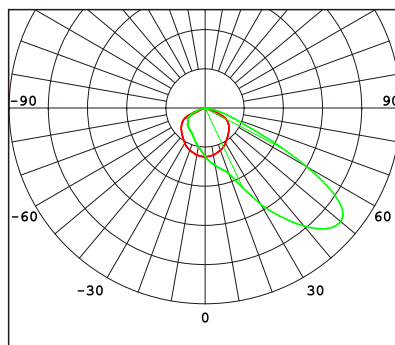
Type III Very Short (44x128° Tilt55°) R01604
