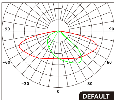
Type II Medium (80x160° Tilt35°) R00802
