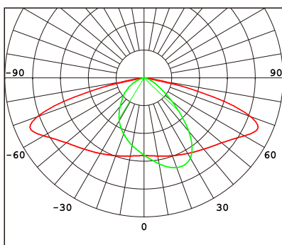
Type II Medium (78x158° Tilt30°) R01611
