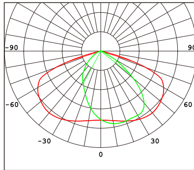
Type III Short (80x148° Tilt30°) R01602
