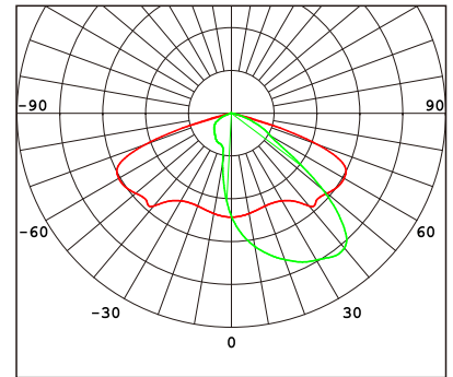
Type II Short (60x150° Tilt40°) R01603
